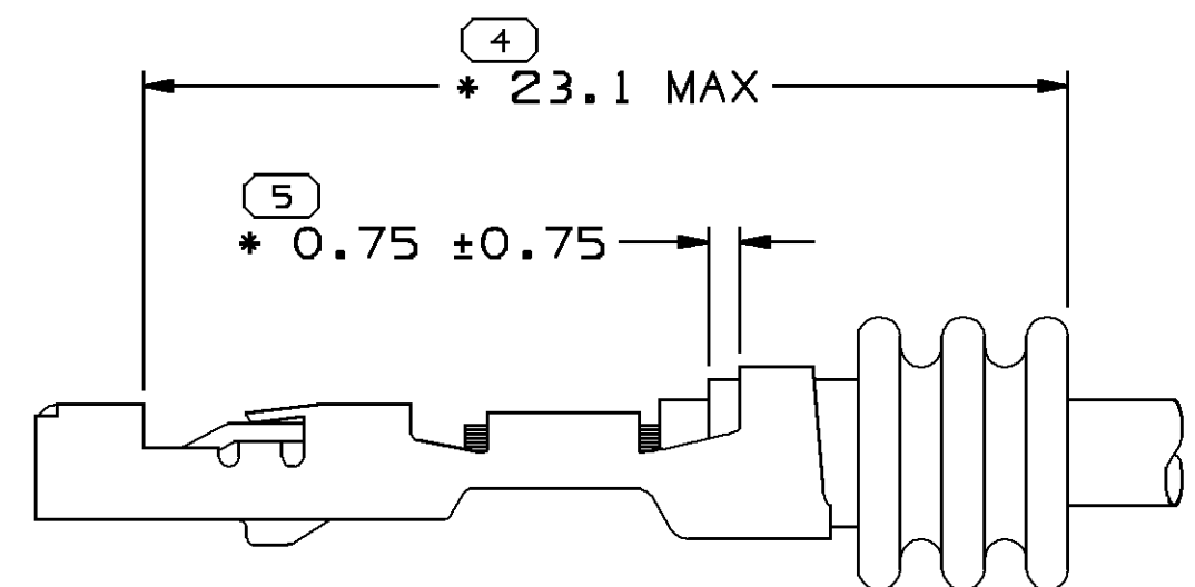
3-RIB SEAL POSITION REF SCALE 5:1
