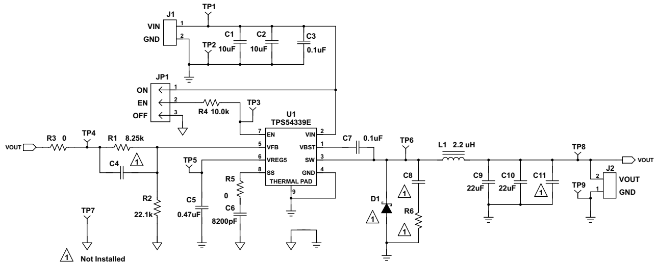
Figure 20. TPS54339EEVM-056 Schematic Diagram
