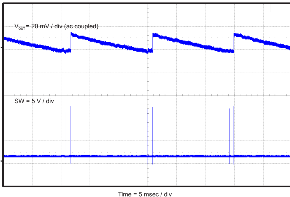
Figure 9. TPS54339EEVM-056 Output Voltage Ripple ( I_{OUT} = 0 \text{ A} )
