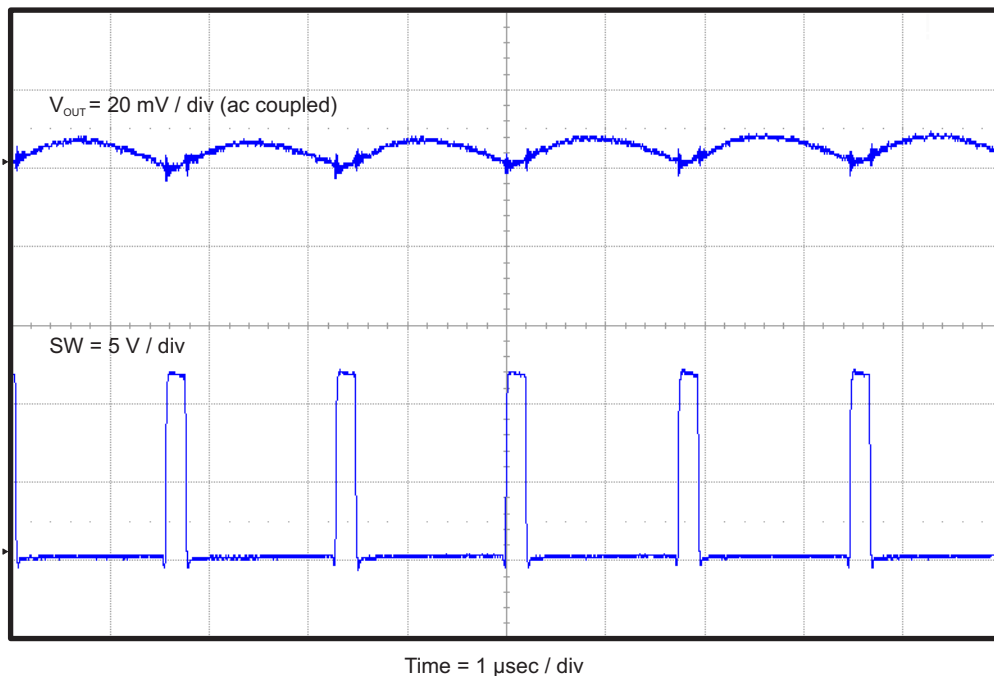
Figure 7. TPS54339EEVM-056 Output Voltage Ripple ( I_{OUT} = 3 \text{ A} )
