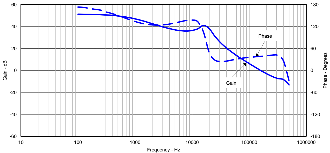
Figure 5. TPS54339EEVM-056 Closed Loop Response
