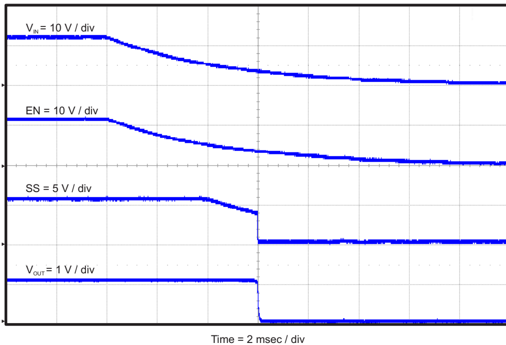
Figure 13. TPS54339EEVM-056 Shut-Down Relative to V_{IN} with SS
