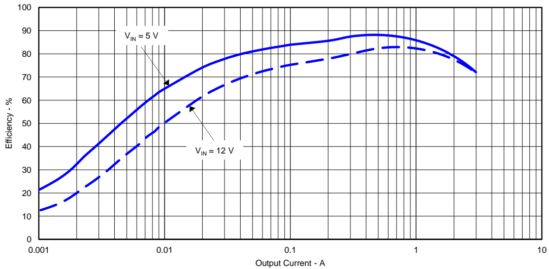
Figure 2. TPS54339EEVM-056 Light-Load Efficiency
