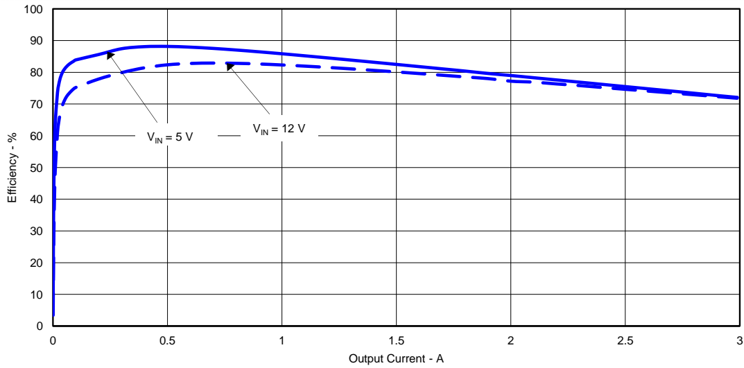
Figure 1. TPS54339EEVM-056 Efficiency
