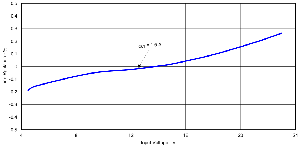
Figure 4. TPS54339EEVM-056 Line Regulation
