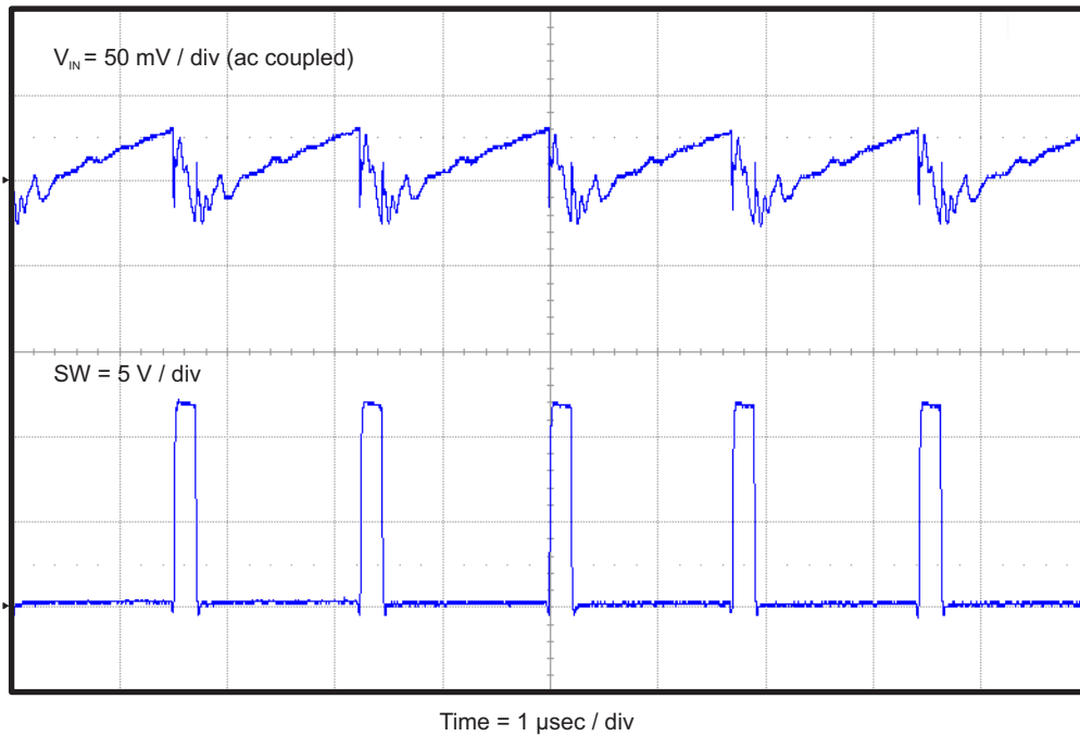
Figure 10. TPS54339EEVM-056 Input Voltage Ripple
