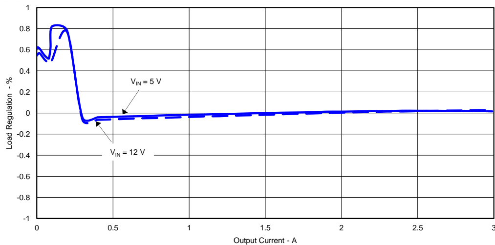
Figure 3. TPS54339EEVM-056 Load Regulation, V_{IN} = 5\text{ V} and V_{IN} = 12\text{ V} .
