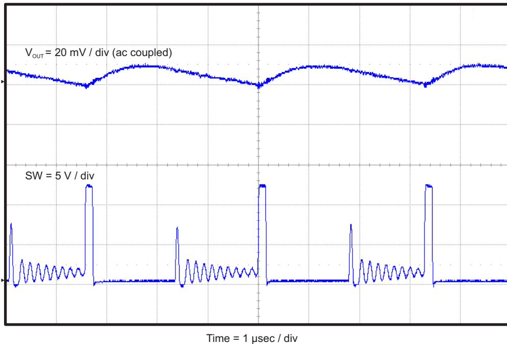
Figure 8. TPS54339EEVM-056 Output Voltage Ripple ( I_{OUT} = 150 \text{ mA} )
