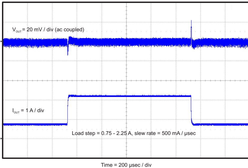
Figure 6. TPS54339EEVM-056 Load Transient Response
