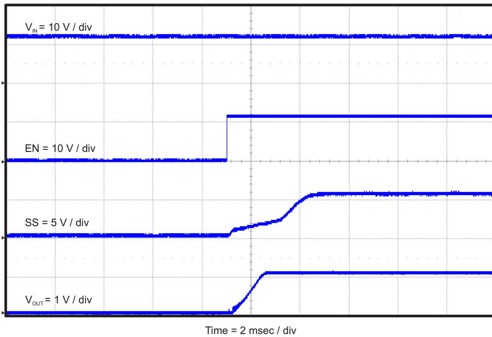
Figure 12. TPS54339EEVM-056 Start-Up Relative to EN with SS
