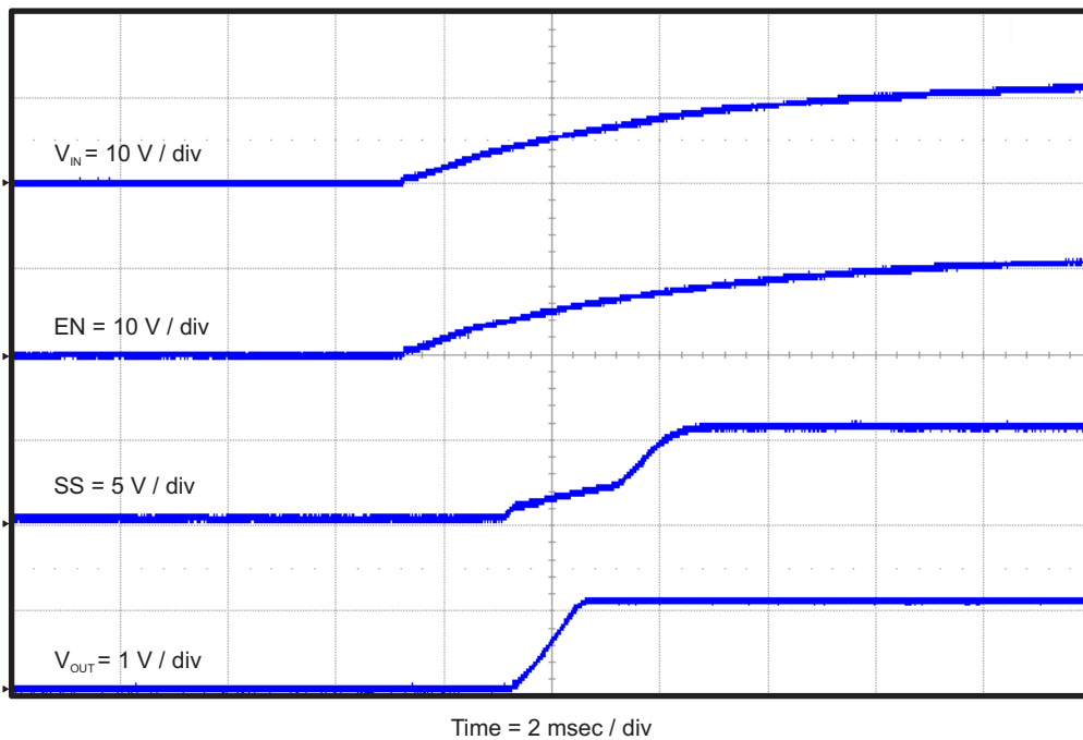
Figure 11. TPS54339EEVM-056 Start-Up Relative to V_{IN} with SS
