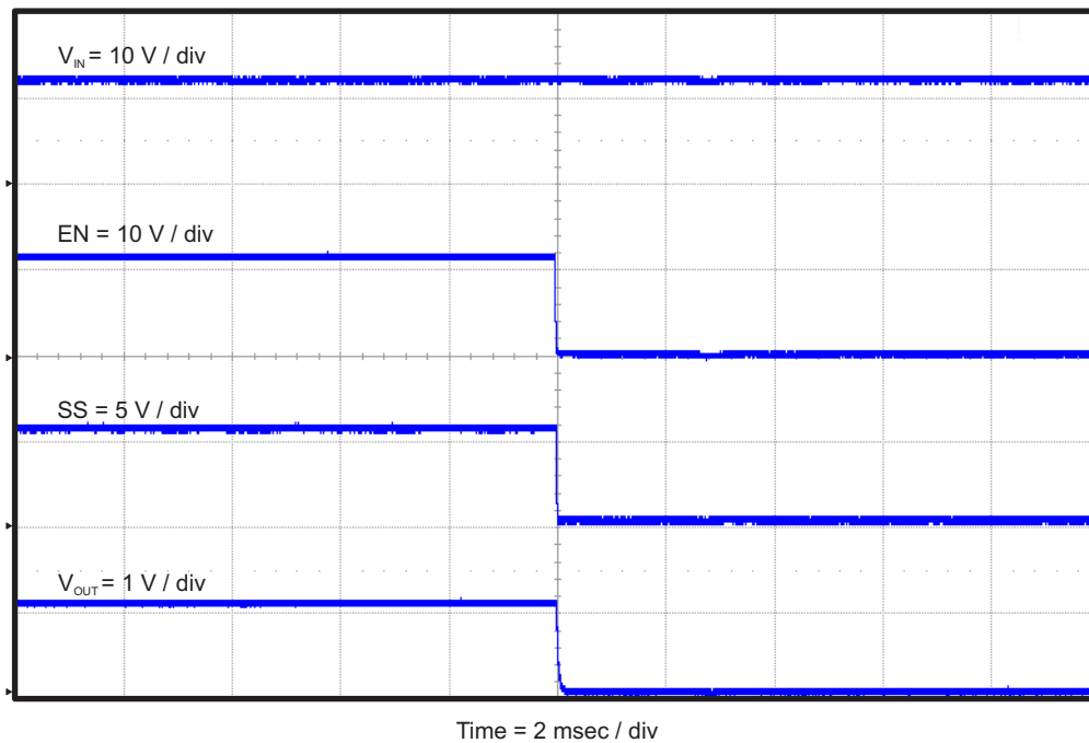
Figure 14. TPS54339EEVM-056 Shut-Down Relative to EN with SS
