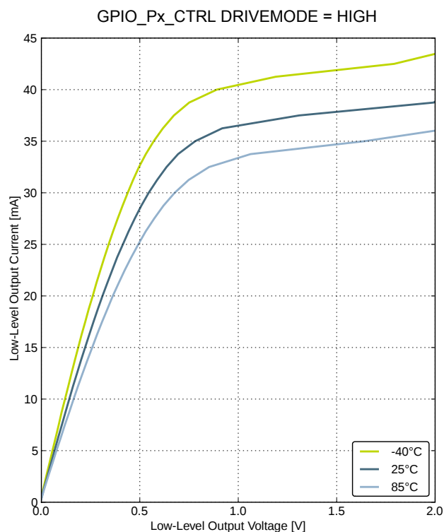
Figure 4.14. Typical Low-Level Output Current, 2V Supply Voltage
