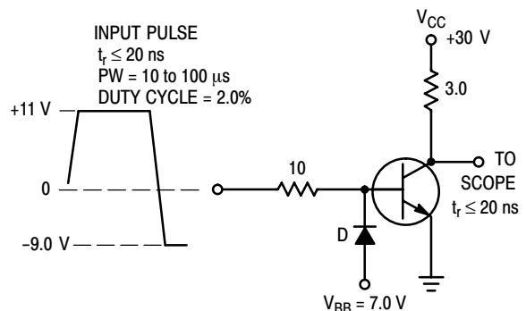
Figure 3. Turn–Off time
