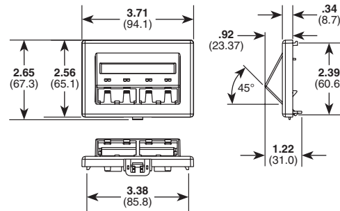
4 Module Space Sloped Herman Miller^ Ethospace Beltline (CFFPEBSL4)
