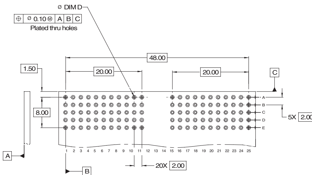
Recommended PCB hole mounting pattern
