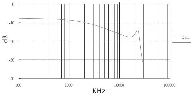
COMMON MODE
