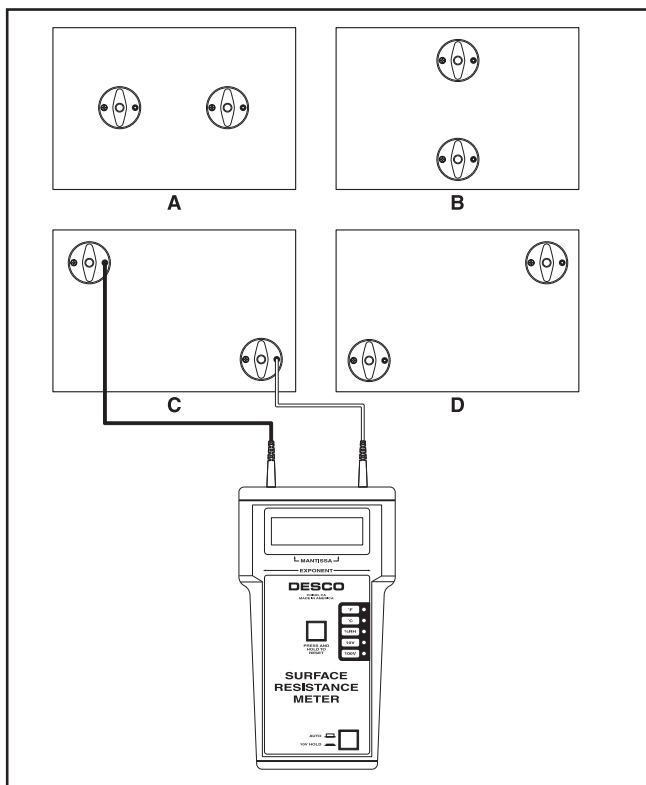
Figure 13. Electrode positions on surface of pad, RTT test.
