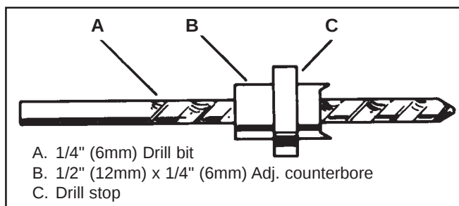
Figure 8. Drill Tool 14242.
