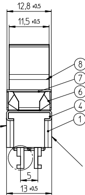
Detail A
