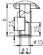
Detail A Scale 5:1
