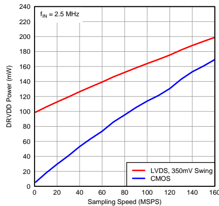
Figure 127. Digital Power LVDS CMOS
