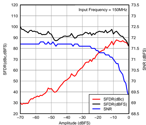
Figure 115. Performance vs Input Amplitude
