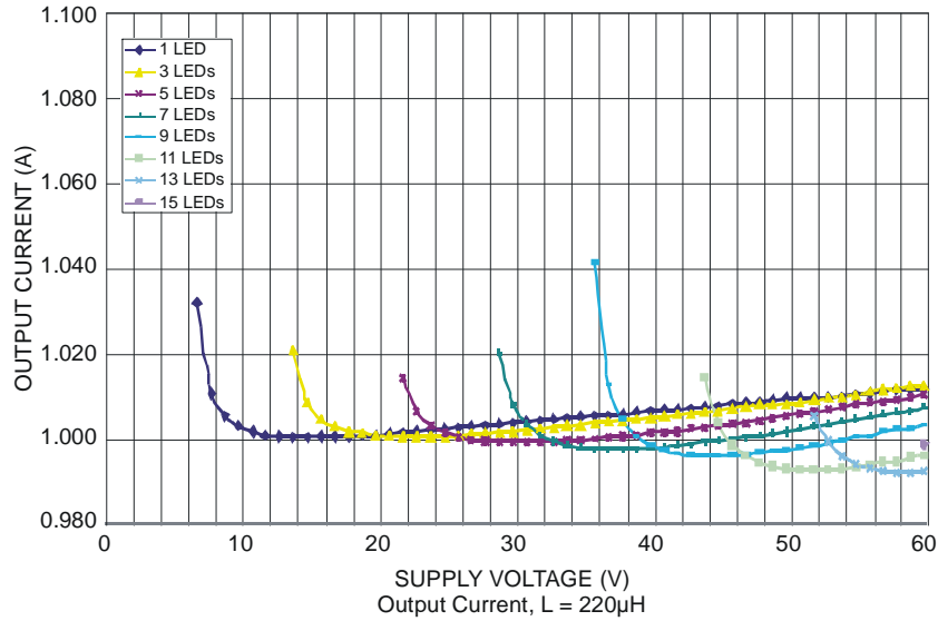
Output Current, L = 220μH
