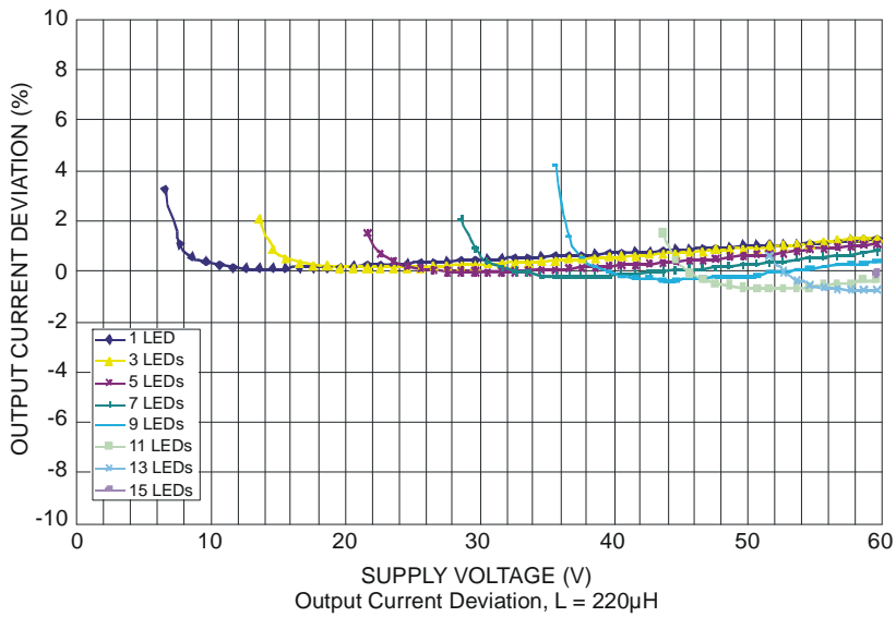
Output Current, L = 220μH
