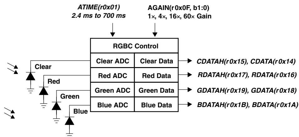
Figure 9. RGBC Operation
