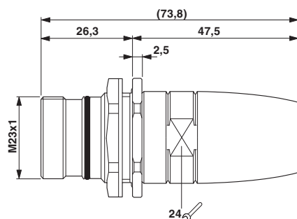
Dimensional drawing
