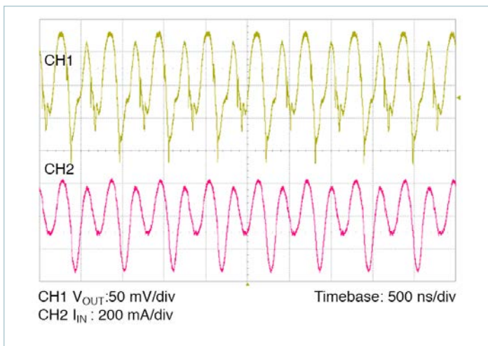
Figure 15 — Full load ripple, 100μF C_{IN} ; No external C_{OUT} . Board mounted module, scope setting : 20MHz analog BW
