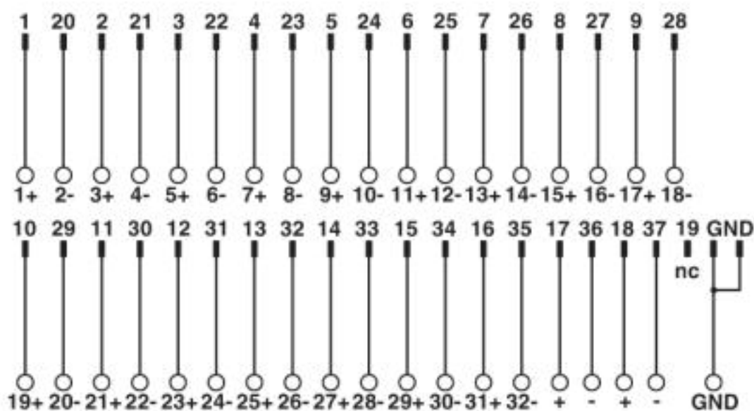
Connection scheme VIP-2/SC/D37SUB/M/SO
