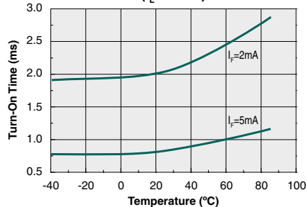
Typical Turn-On vs. Temperature ( I_L=70\text{mA} )
