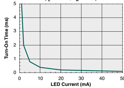
Typical Turn-On vs. LED Forward Current ( I_L=70\text{mA} , T_A=25^\circ\text{C} )
