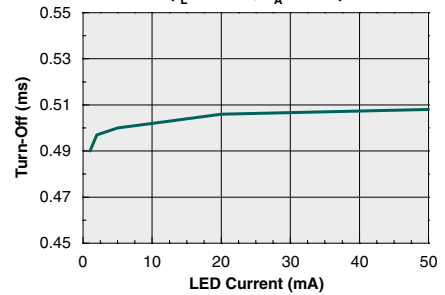
Typical Turn-Off vs. LED Forward Current ( I_L=70\text{mA} , T_A=25^\circ\text{C} )
