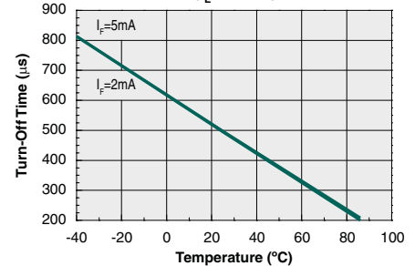
Typical Turn-Off vs. Temperature ( I_L=70\text{mA} )
