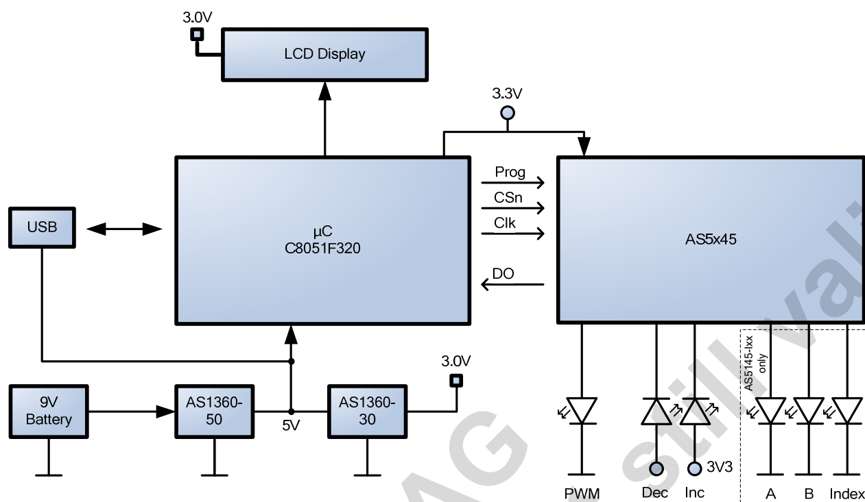
Figure 9: AS5x45 Blockdiagramm
