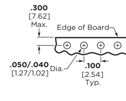
Recommended Mounting Hole Pattern for .062 [1.57] Thk. PC Board (Solder Side of Board Shown)
