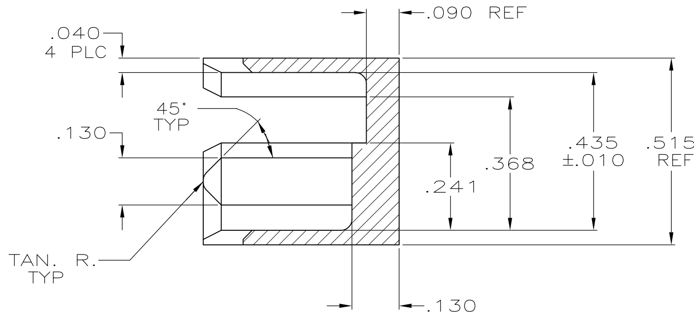
SECTION X-X
