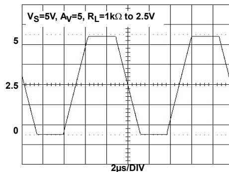
FIGURE 26. OUTPUT SWING
