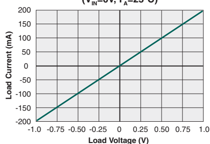
Typical Load Current vs. Load Voltage ( V_{IN} = 0V, T_A = 25^{\circ}\text{C} )
