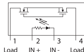
CPC1219 Pinout
