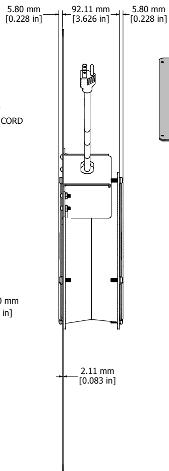
ASSEMBLY - VIEW FROM SIDE
