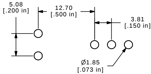
P.C. MOUNTING
