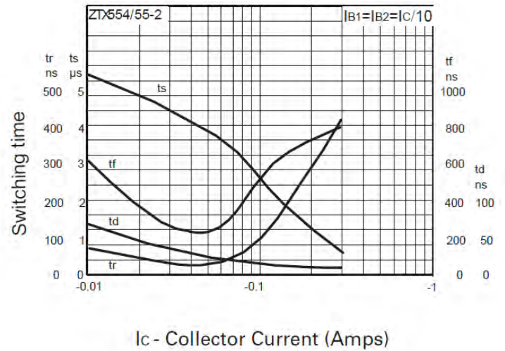
Switching Speeds
