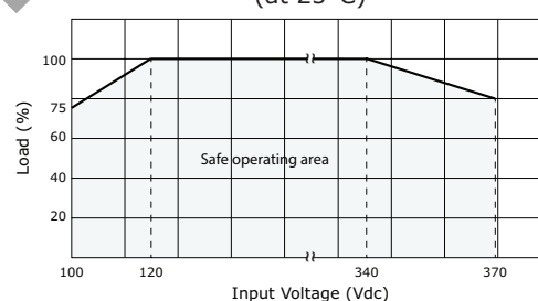
load vs. input voltage (Vdc) (at 25°C)
