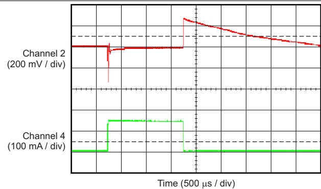
Channel 2 = V_{\text{OUT}} , channel 4 = I_{\text{OUT}} , V_{\text{IN}} = 2.7\text{ V}
