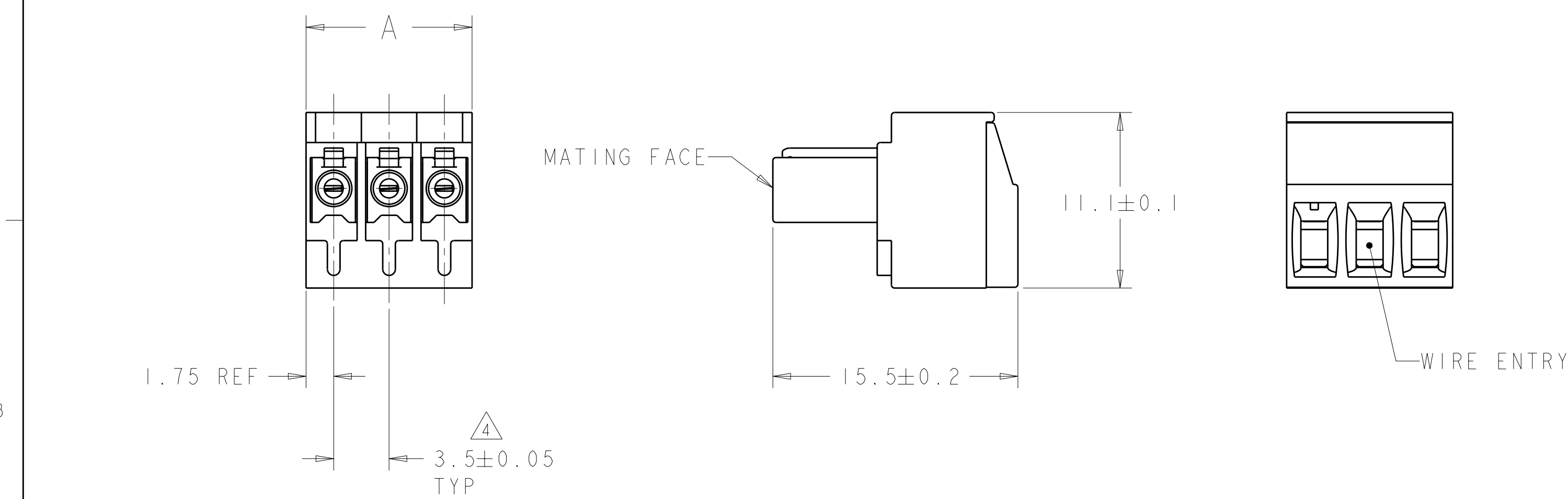
796693-3 AS SHOWN
