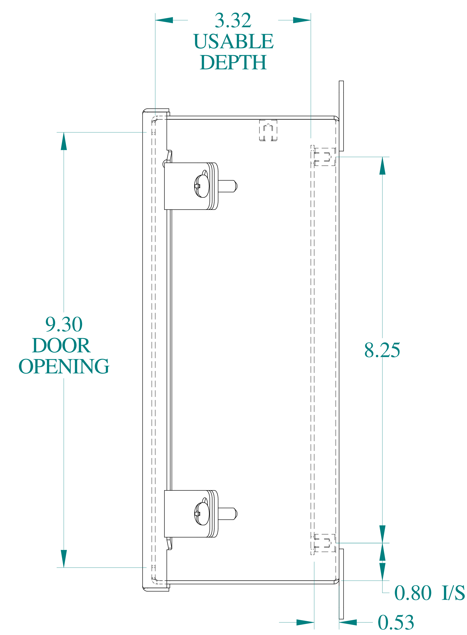
SIDE VIEW
