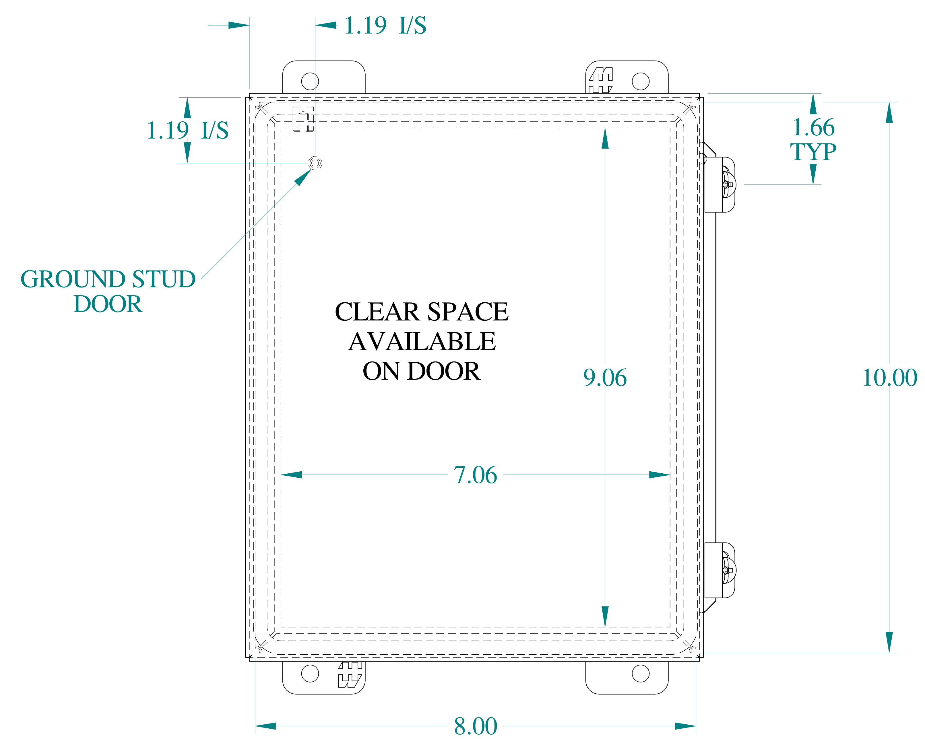
FRONT VIEW
