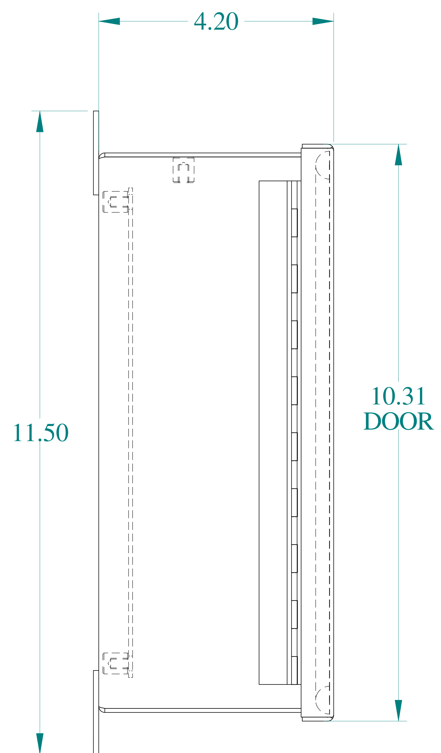
SIDE VIEW
