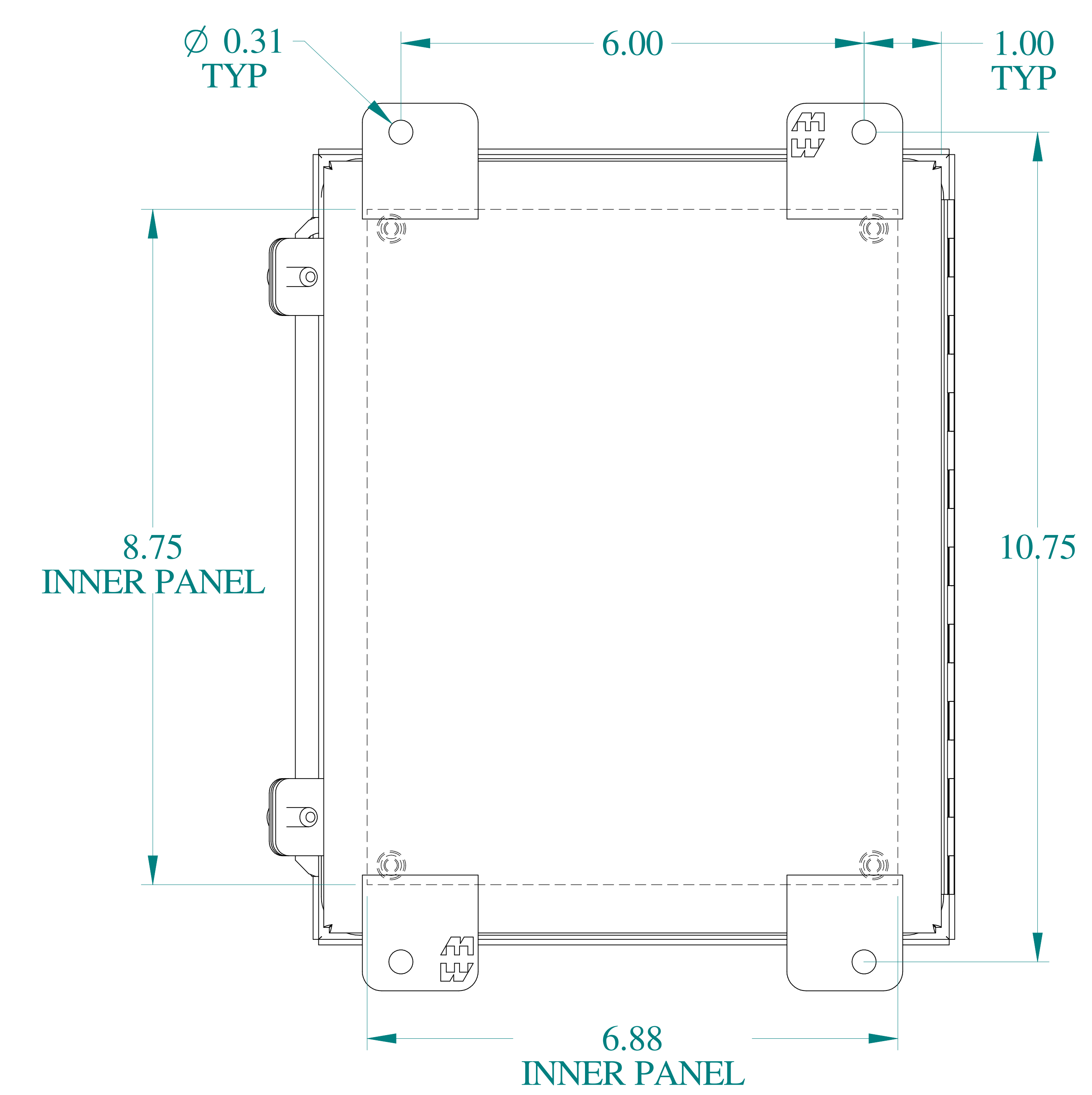
BACK VIEW
