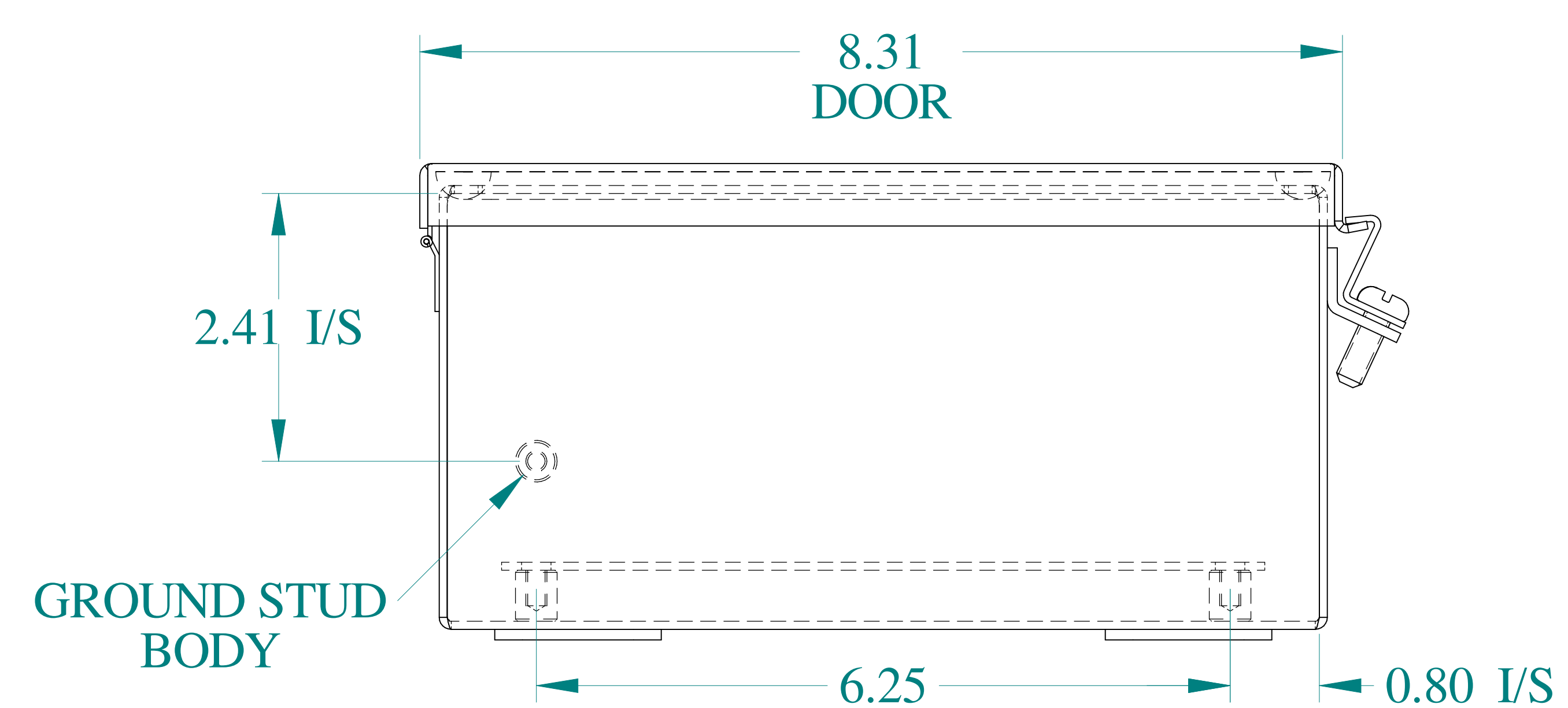
BOTTOM VIEW
