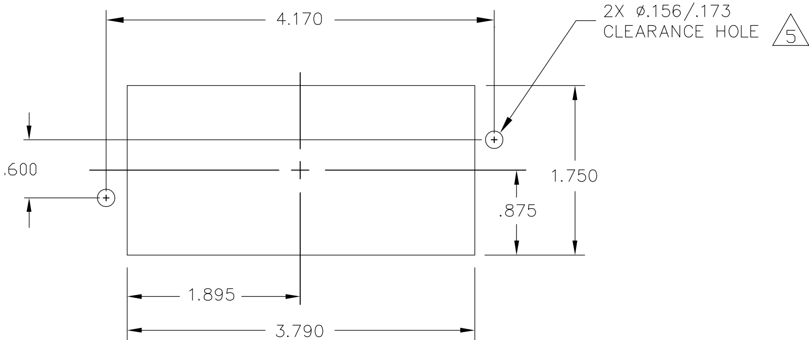
PIN PANEL MOUNT CUTOUT SCALE: NONE
