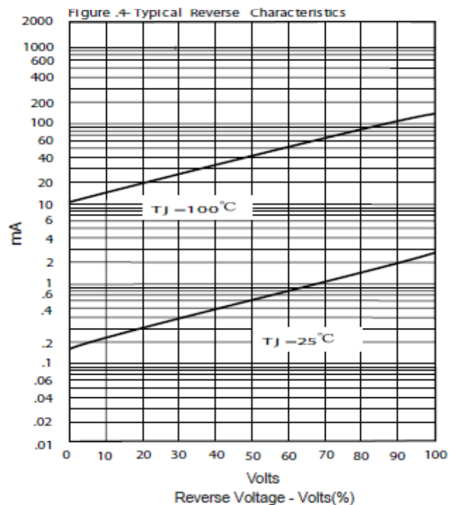
Instantaneous Reverse Leakage Current - mA
