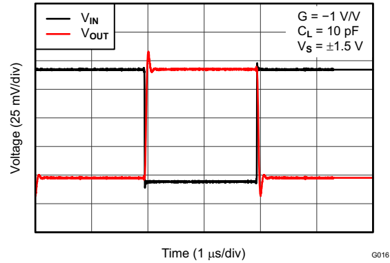
Time (1 \mu\text{s}/\text{div} ) G016 Figure 20.
