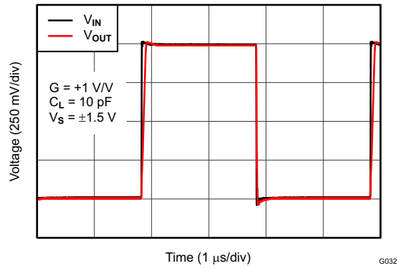
Time (1 \mu\text{s}/\text{div} ) G032 Figure 22.
