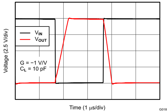
Time (1 \mu\text{s}/\text{div} ) G018 Figure 23.
