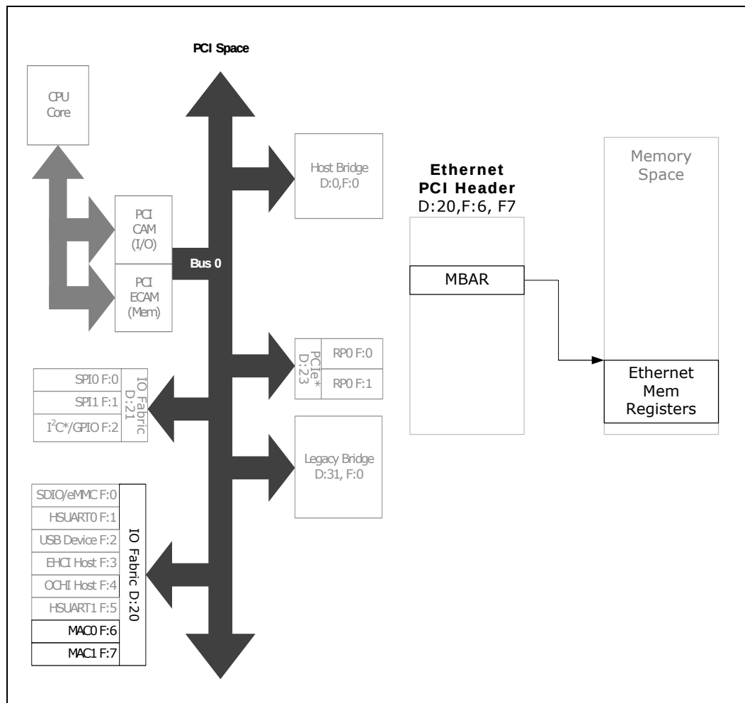
Figure 28. Ethernet Register Map
