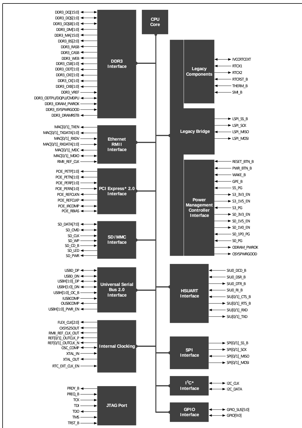
Figure 3. Signals In Default System Pin List
