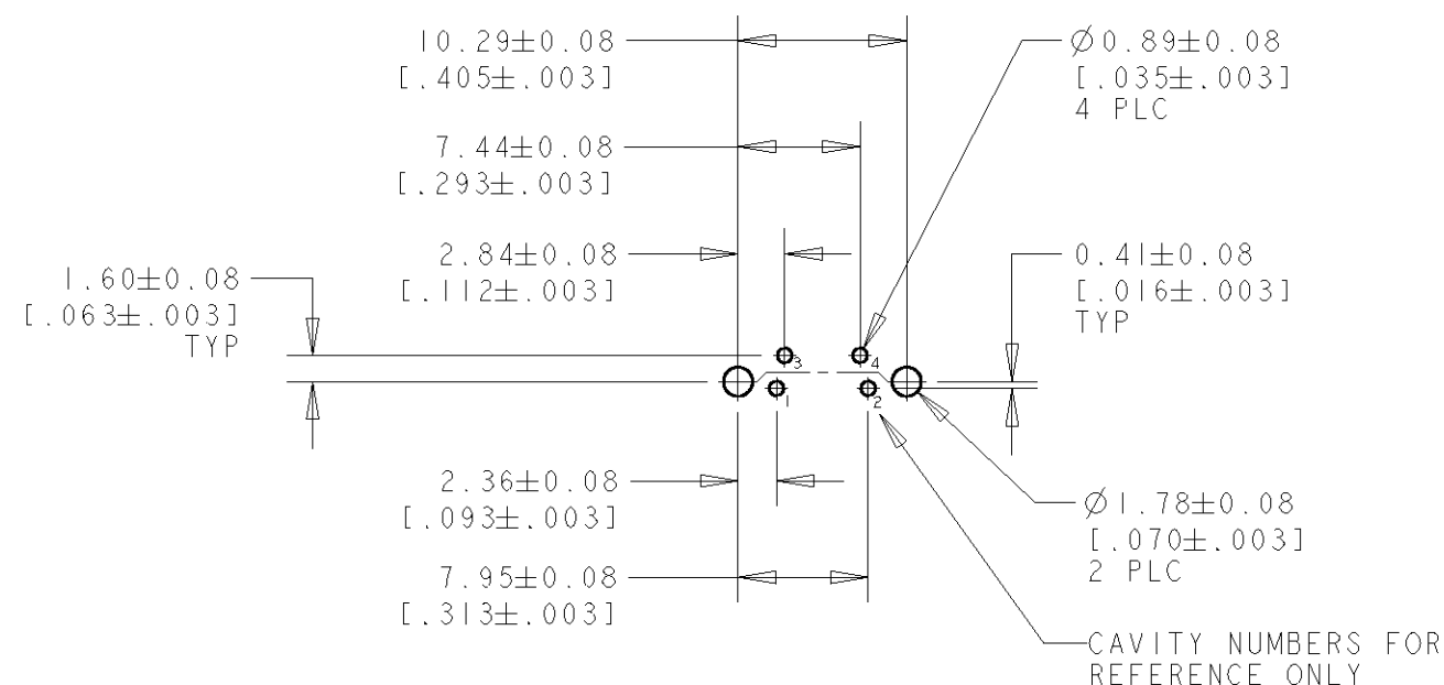
RECOMMENDED PC BOARD LAYOUT BOTTOM VIEW
