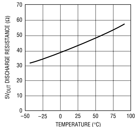
5V OUT Discharge Resistance vs Temperature
