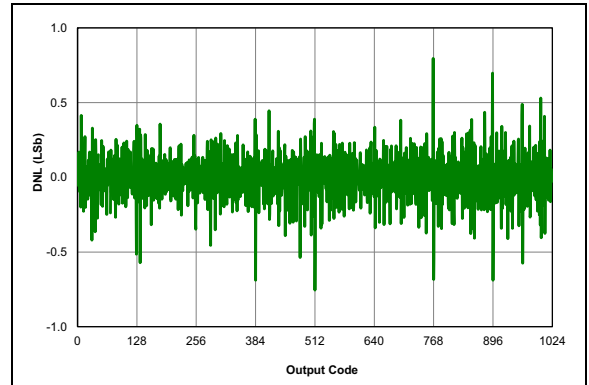
FIGURE 29-63: ADC 10-bit Mode, Single-Ended DNL, V_{DD} = 3.0V , T_{AD} = 1\ \mu\text{S} , 25^\circ\text{C} .
