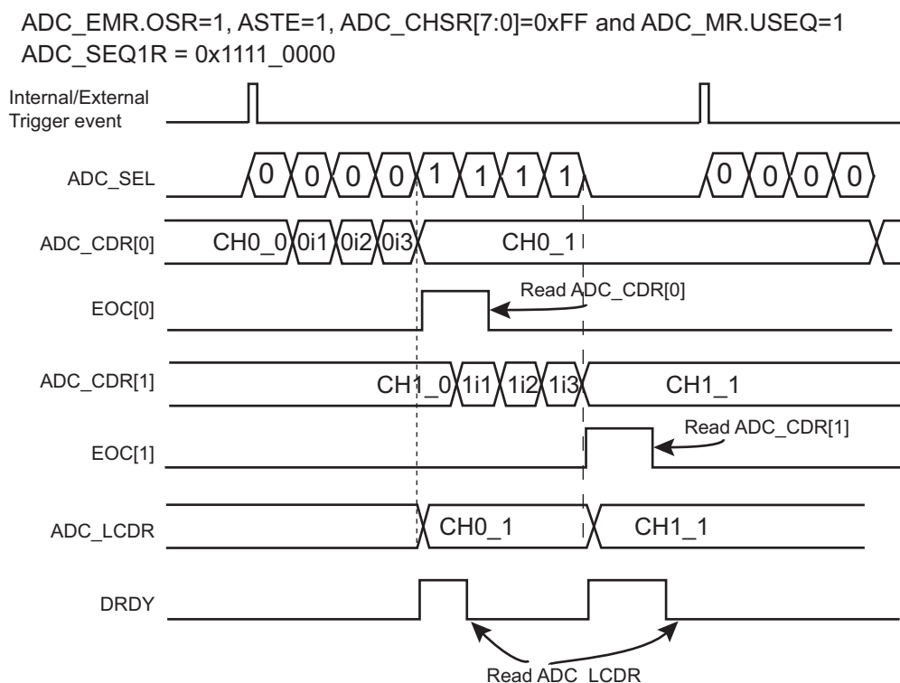
Figure 40-11. Digital Averaging Function Waveforms on Single Trigger Event, Non-interleaved
