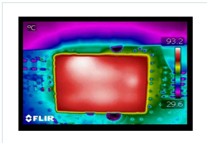
Figure 10 — Thermal image ( V_{IN} = 24V , I_{OUT} = 10A , CR, OLFM evaluation PCB)
