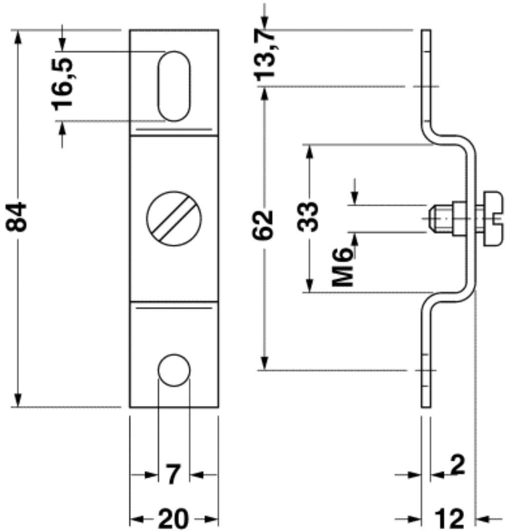
Dimensional drawing
