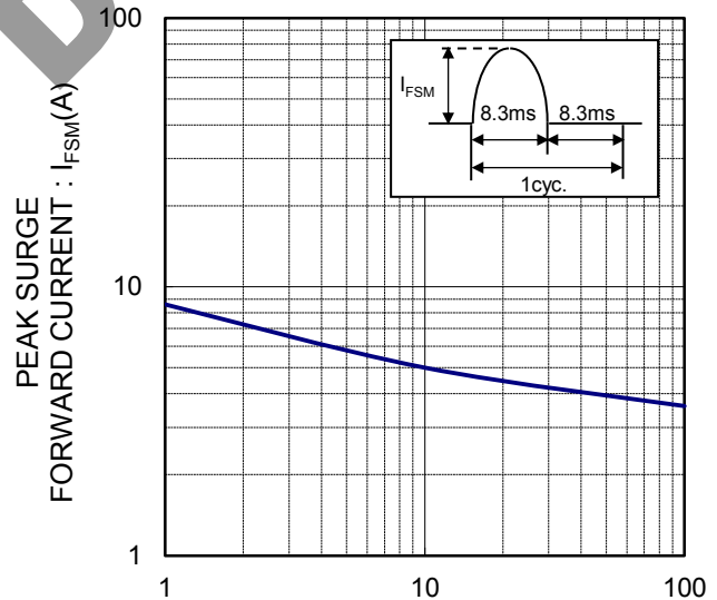
IFSM-CYCLE CHARACTERISTICS
