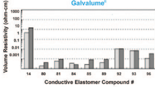
Graph 2 Galvalume®
