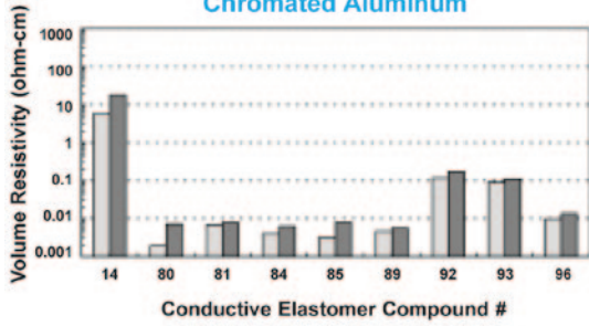
Graph 1 Chromated Aluminum
