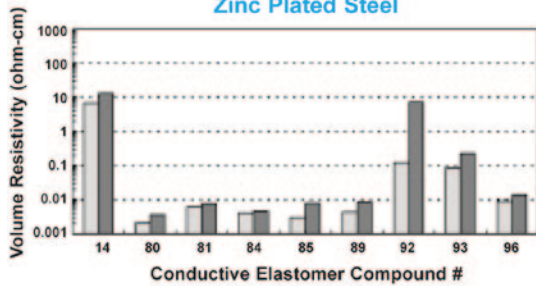
Graph 5 Zinc Plated Steel
