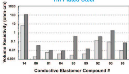
Graph 3 Tin Plated Steel
