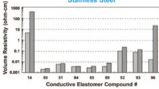
Graph 4 Stainless Steel
