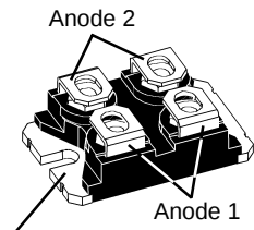
Common cathode
