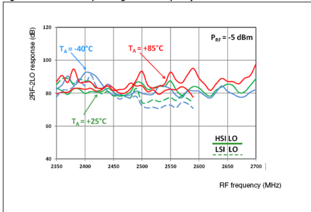
Figure 6. 2RF-2LO response against RF frequency
