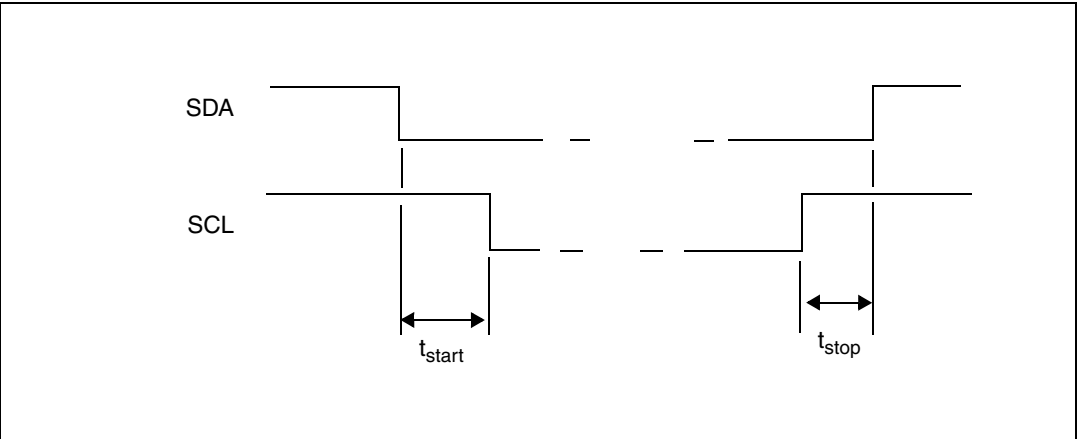
Figure 18. I 2 C START and STOP timing waveforms
