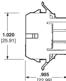
Plug Rear
