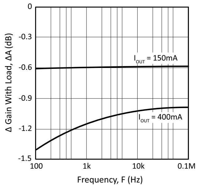
Figure 19: Loading Effects
