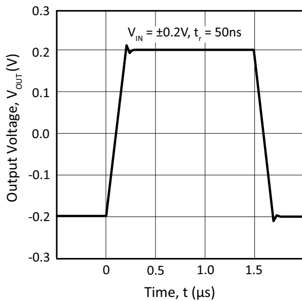
Figure 18: Pulse Response
