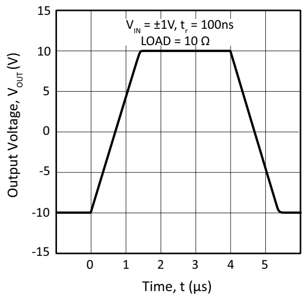
Figure 19: Loading Effects
