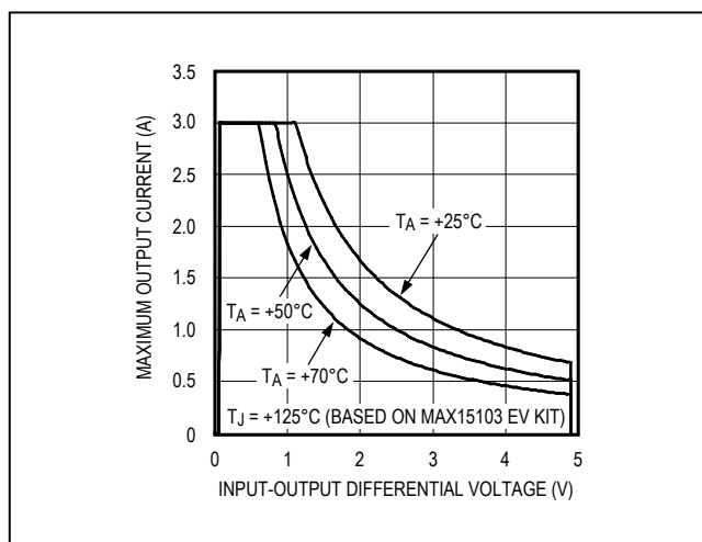
Figure 1. Maximum Output Current Curves
