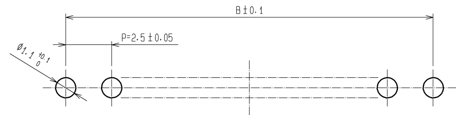
RECOMMENDED PATTERN(5:1)
