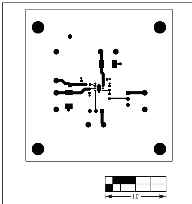
Figure 3. MAX9943 EV Kit PCB Layout—Component Side
