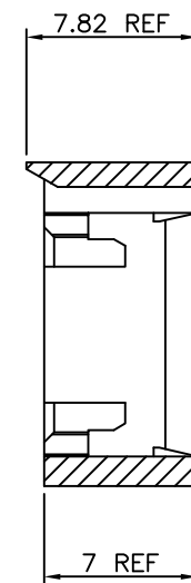
SECTION B-B
