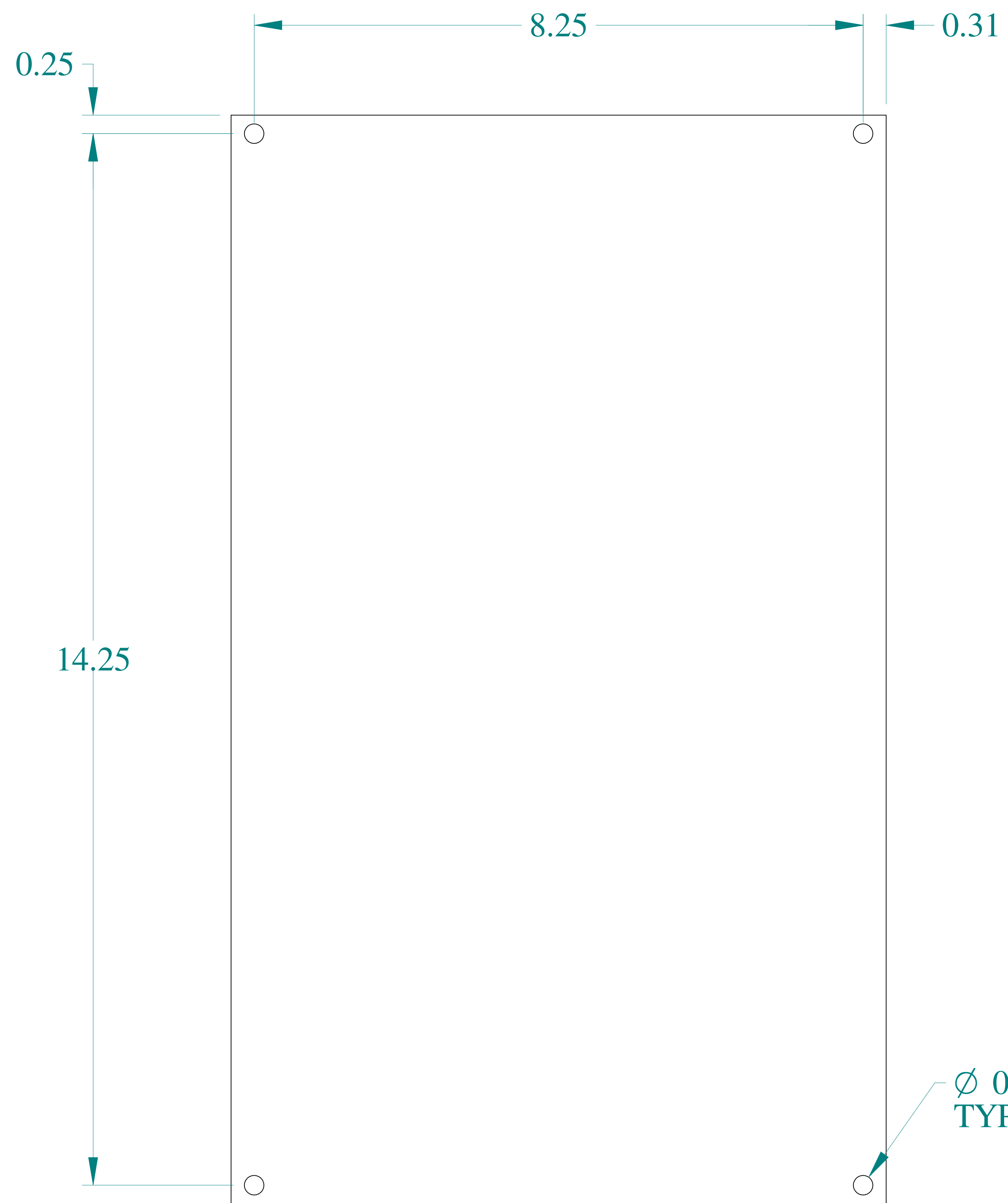
FRONT VIEW
