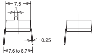
Raised actuator
